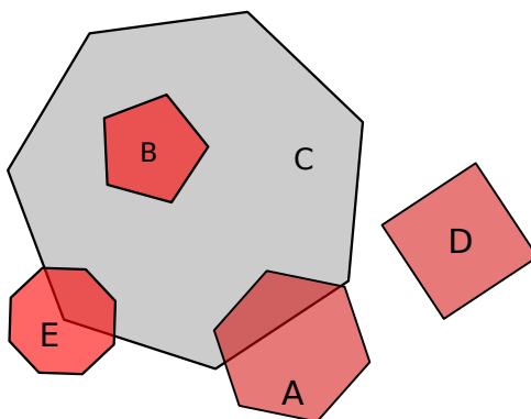
Figure 167: Example image used for polygon/polygon collision detection
